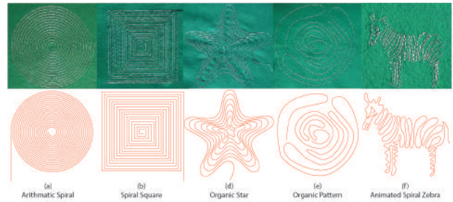
Figure 4: Examples of geometric, organic and animated spiral patterns for soft speakers and vibro-haptic actuators
