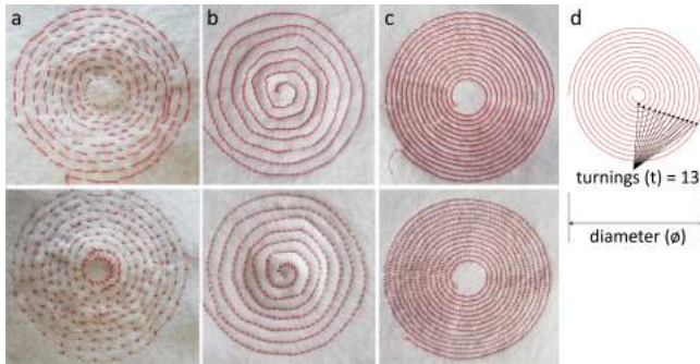
Figure 3: Soft Speakers using: a) hand-embroidery (1-4 hours); b) mechanical sewing machine (20-40 min); and c) digital sewing machine (2-4 min); and d) the arithmetic spiral pattern
